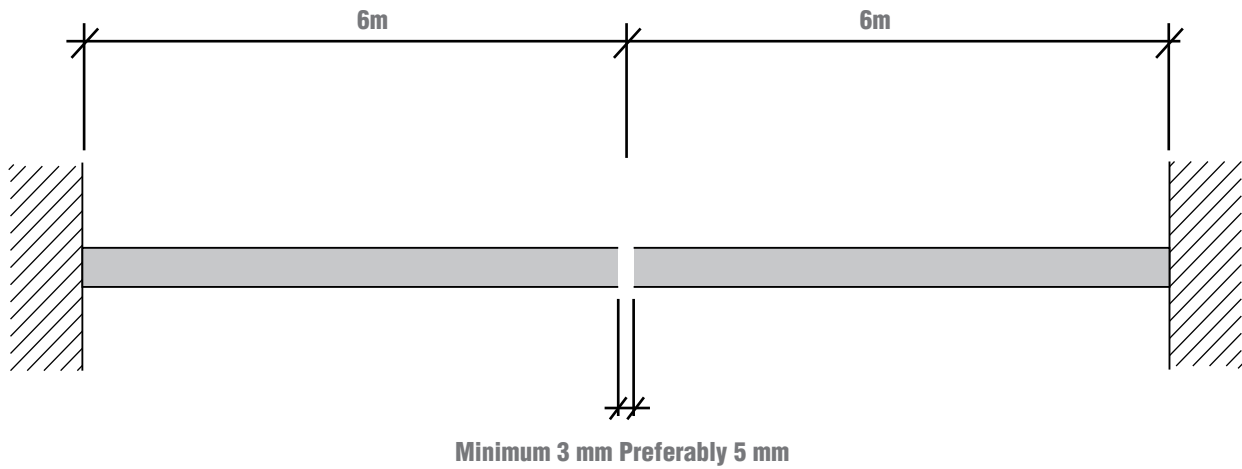
Figure 3: Leaving space between box steel profiles
