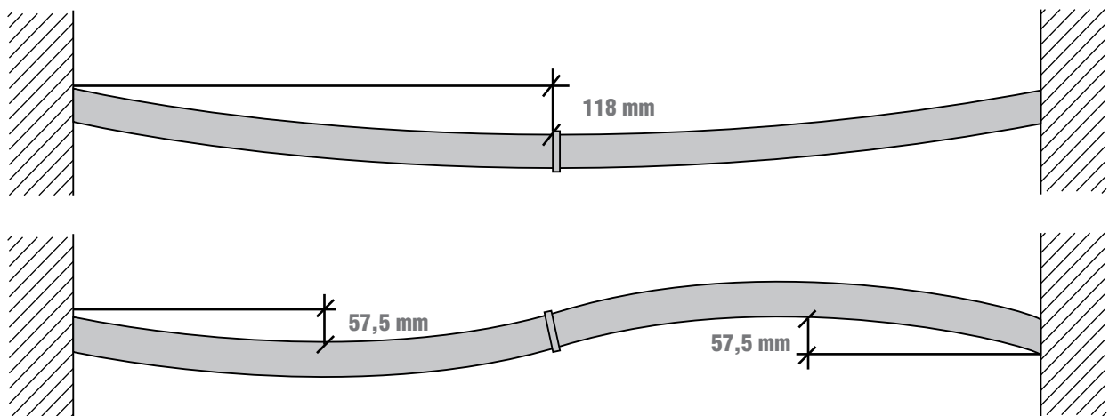
Figure 2: Concave or convex bending
